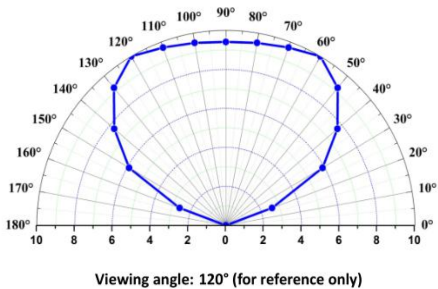
Typical Emission Distribution Curve
